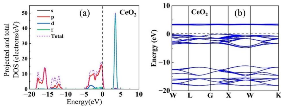
Fig. 2. a): The projected and total density of states (DOSs). b): The band structure of the pristine \text{CeO}_2 at 0 \text{ GPa} .
